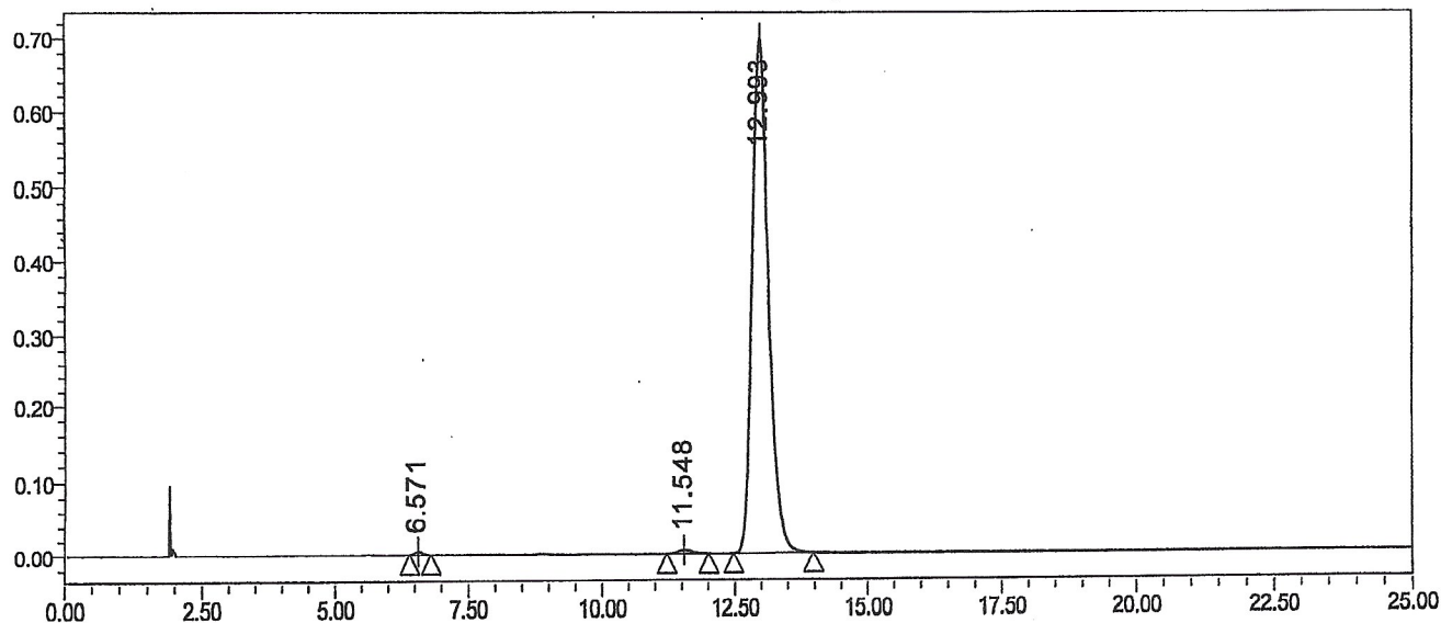
Auto-Scaled Chromatogram
